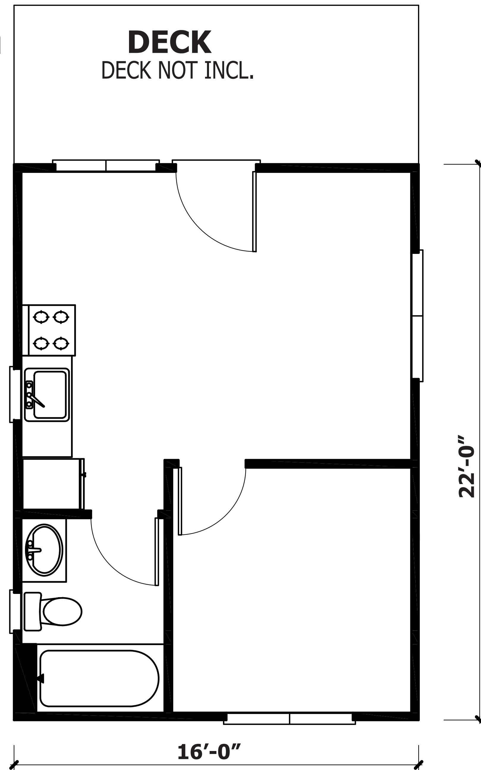
FLOOR PLAN 352 sq. ft.
