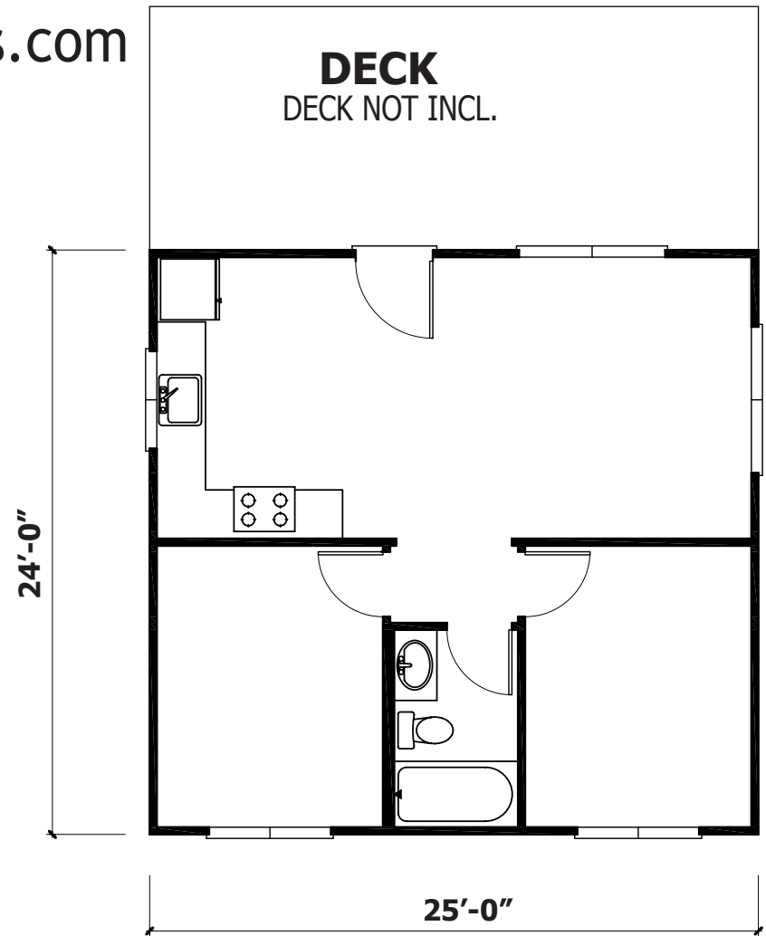
FLOOR PLAN
