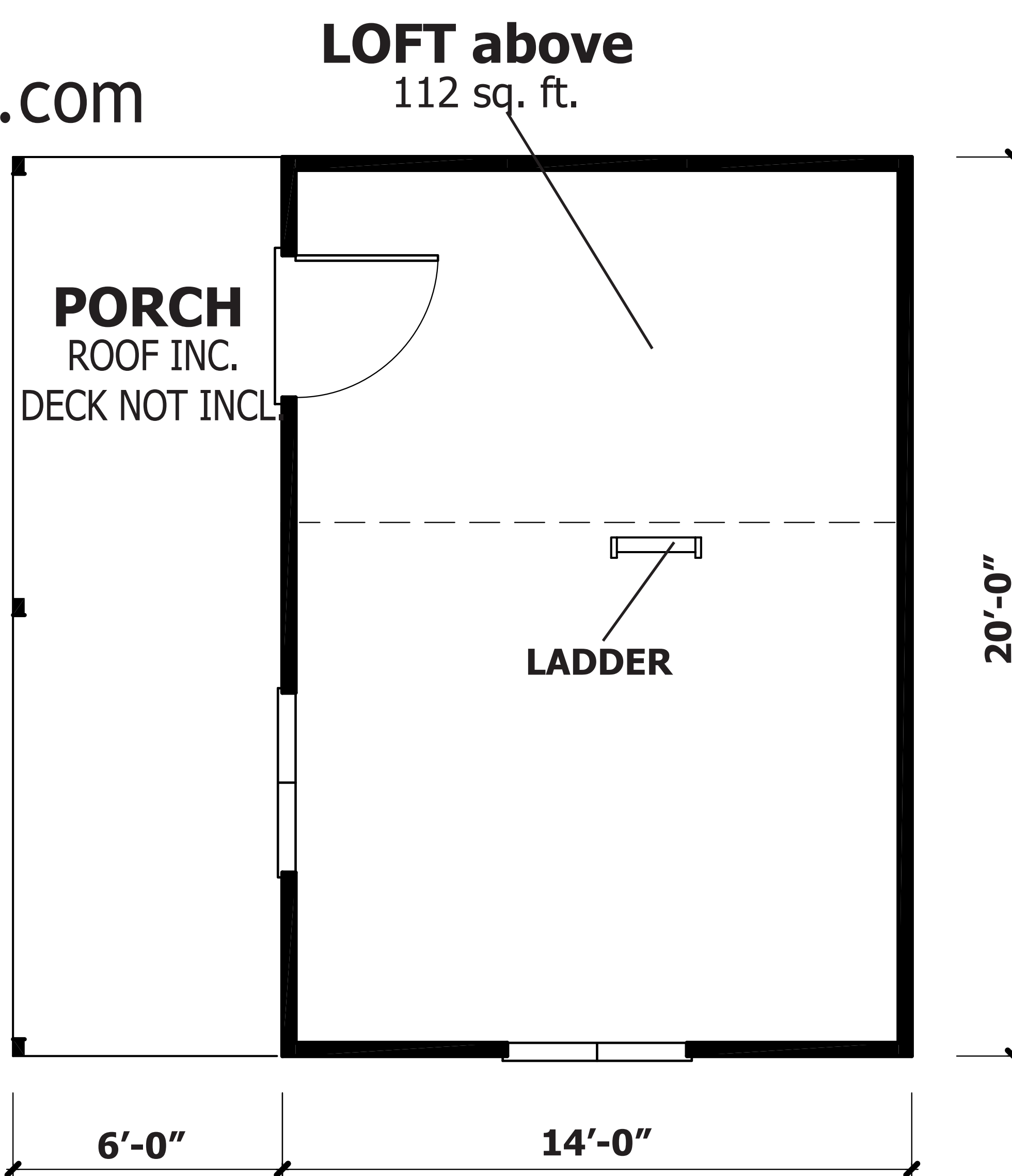
FLOOR PLAN 280 sq. ft.
